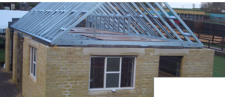
roof system
